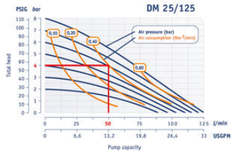
Pump - Aluminium, Gçuğm, Aluminium + PTFE
