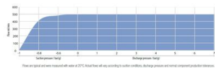
Performance curve
