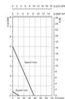
Performance charts*
