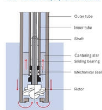
F 310 - The small drum pump with mechanical seal
