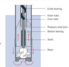
F 314/FP 314 - The small sealless drum pump
