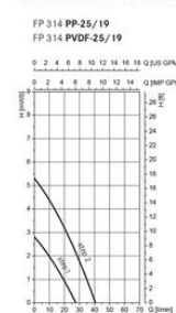
Performance charts*
