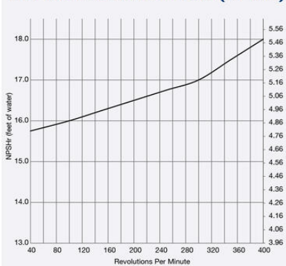
Net Positive Suction Head (NPSHr)
