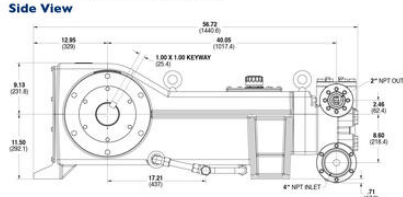
Threaded Version Inches (mm)
