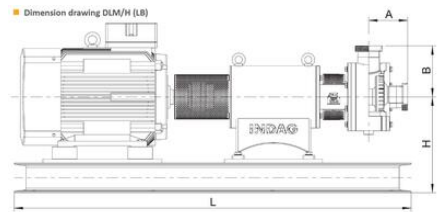
■ Dimension drawing DLM/H (LB)
