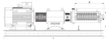
■ Dimension drawing of DLM/S (LB)
