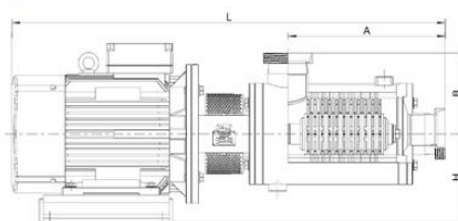
■ Dimension drawing of DLM/S (KB)
