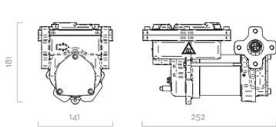
Dimensions expressed in millimeters
