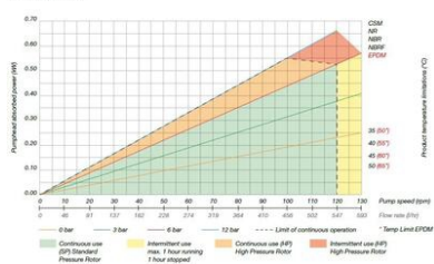
Performance curve
