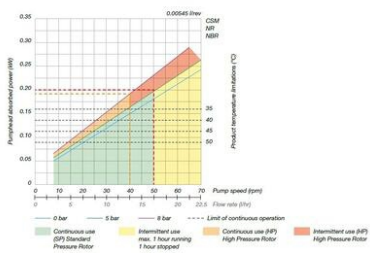
Performance curve
