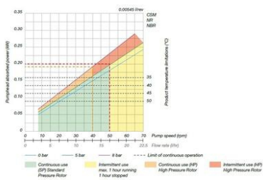
Performance curve
