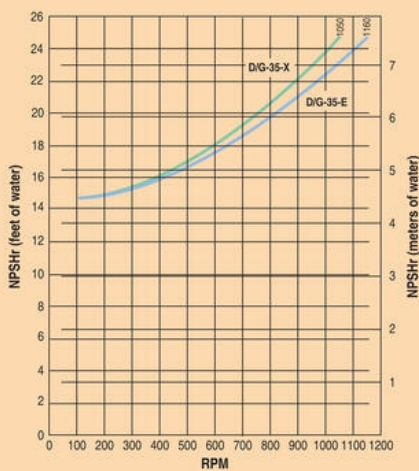
Net Positive Suction Head (NPSHr)
