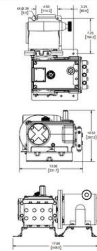
MTS Low Pressure with Manual-Adjust Gear Reducers
