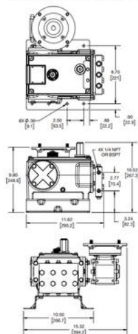
MTS Low Pressure with Fixed-Ratio Gear Reducers
