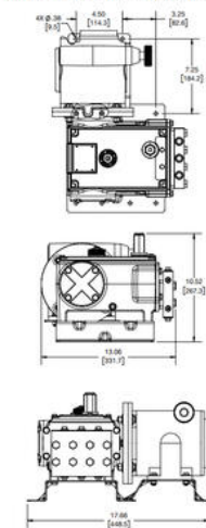
MTS Low Pressure with Manual-Adjust Gear Reducers
